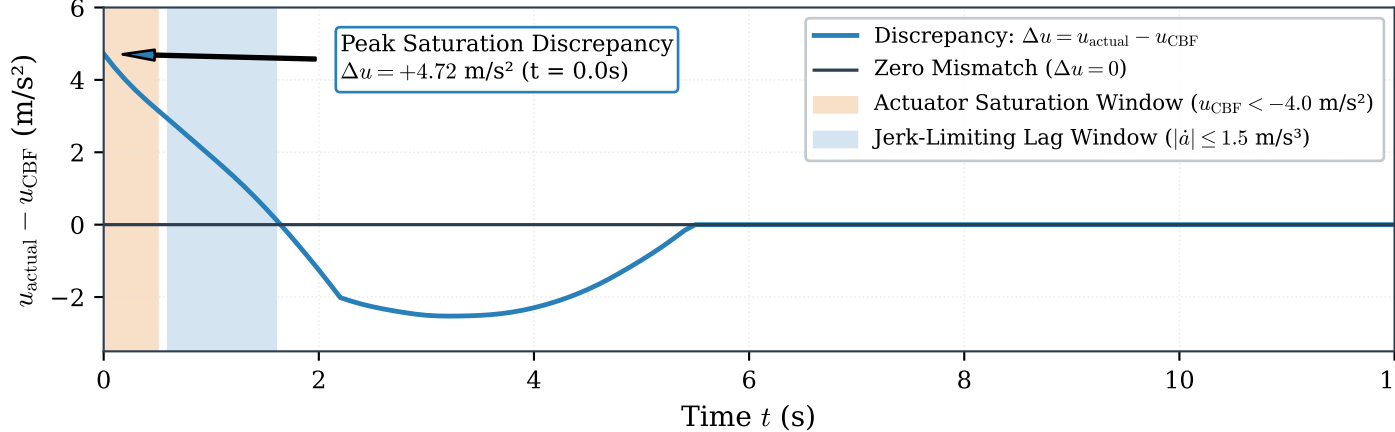
(b) Trajectory 51: Actuator Saturation & Jerk Rate-Limiting
