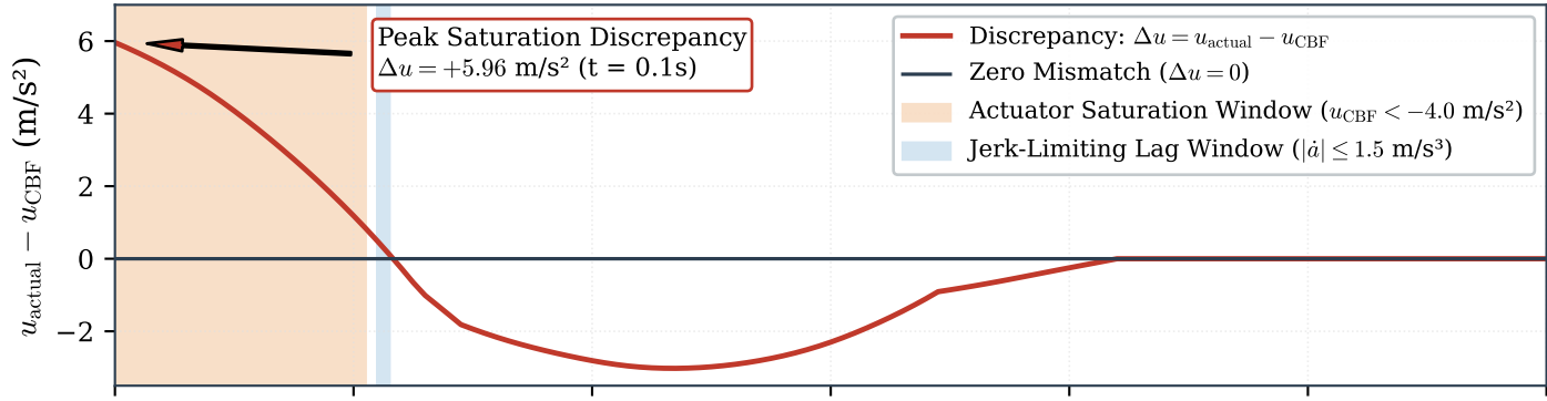
(b) Trajectory 51: Actuator Saturation & Jerk Rate-Limiting
